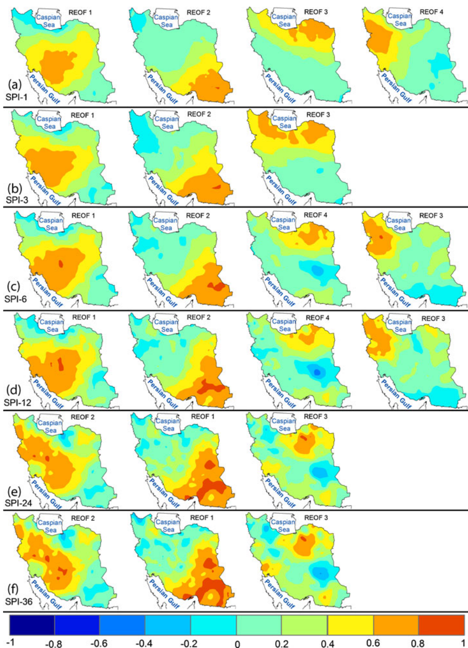
Fig. 4 As in Fig. 2 but for GPCC precipitation data with 0.5^\circ resolution
