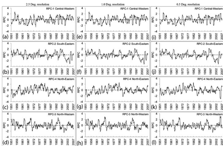
Fig. 5 Rotated principal component score time series (RPCs) obtained for the SPI on 12-month time scale at different GPCP spatial resolutions and associated with the rotated loadings shown in Figs. 2, 3 and 4
