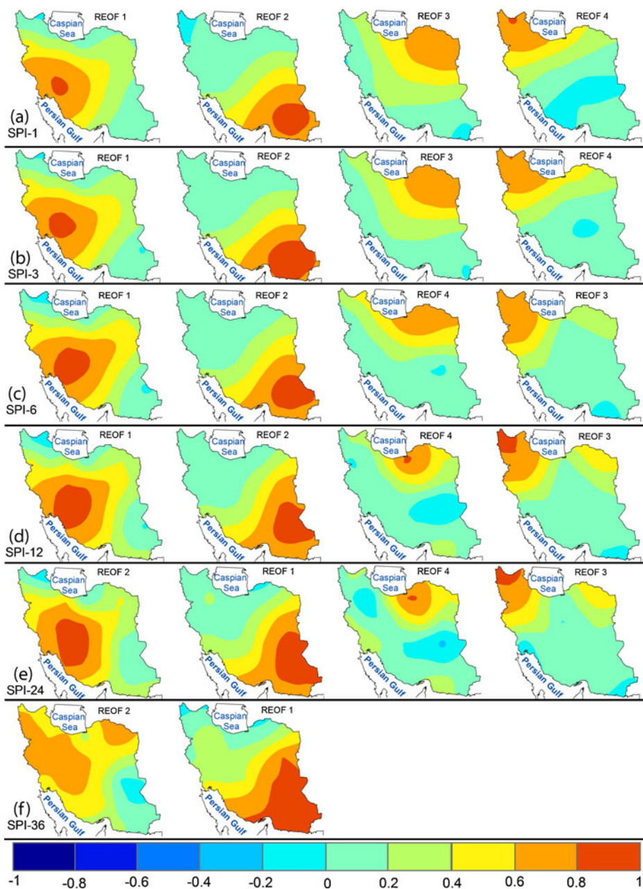
Fig. 2 Varimax rotated loadings (REOFs) of the SPI on different time scales computed using GPCP precipitation data with 2.5° resolution. Sub-regions are identified by loading values greater than 0.6–0.7 (orange and red areas)
