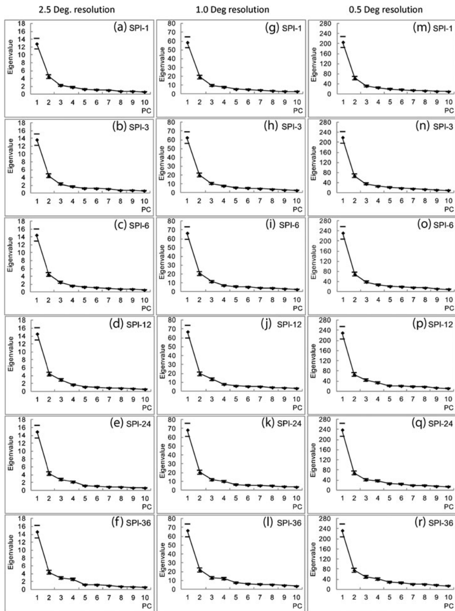
Fig. 1 First ten eigenvalues with the corresponding errorbars at 95 % confidence level resulting from the PCA applied to the SPI computed on different time scales and GPCC spatial resolutions
