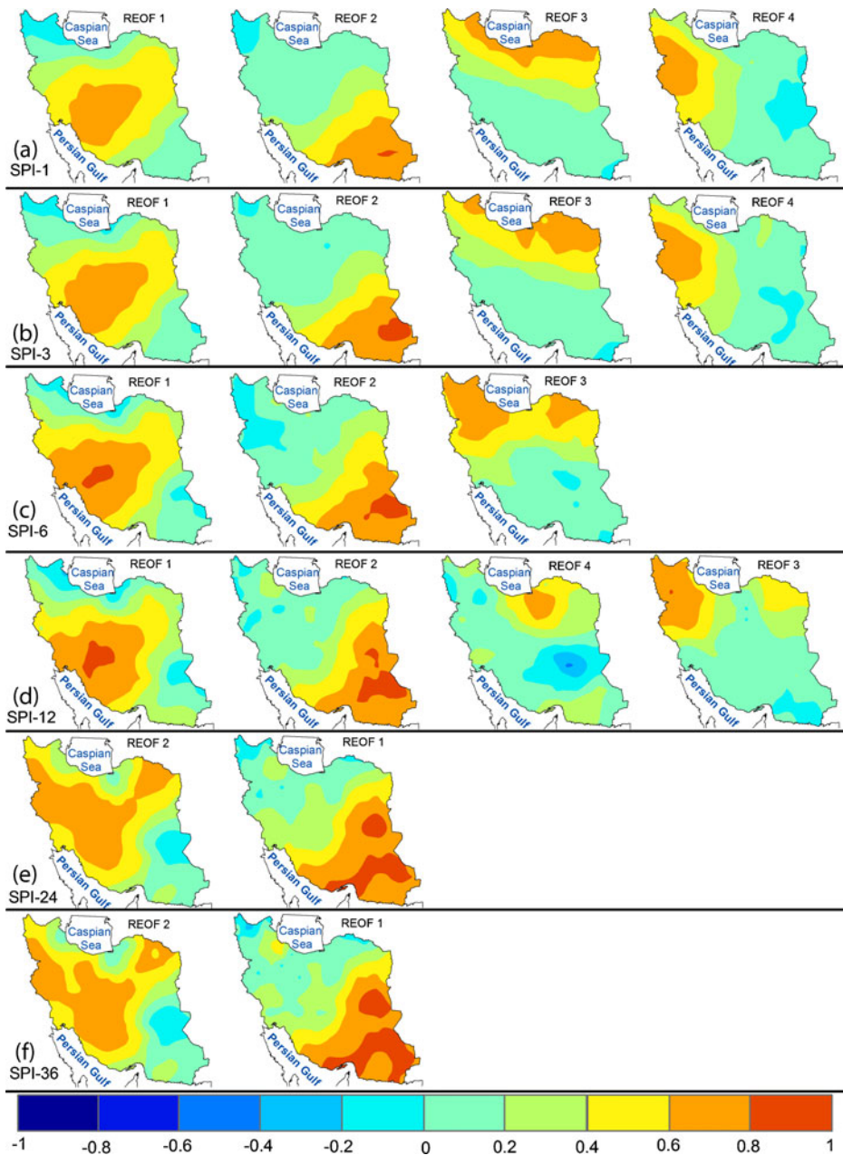
Fig. 3 As in Fig. 2 but for GPCC precipitation data with 1^\circ resolution
